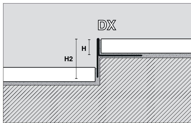
TPC148-11-DX
