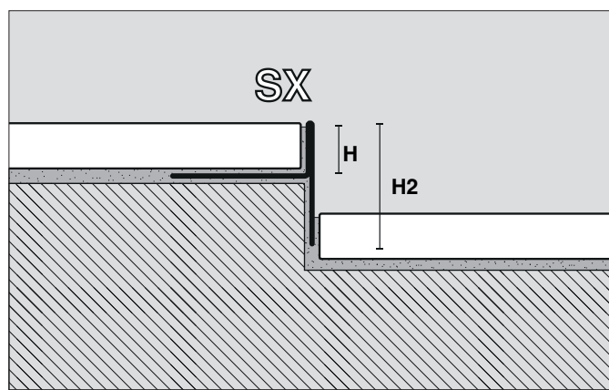
TPC148-11-SX
